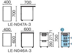
LE-N047A-3 LE-N046A-3
