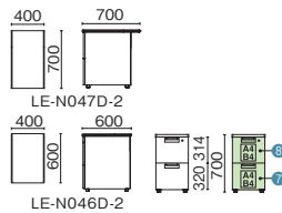
LE-N047D-2 LE-N046D-2
