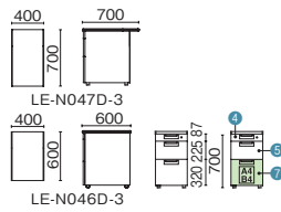
LE-N047D-3 LE-N046D-3
