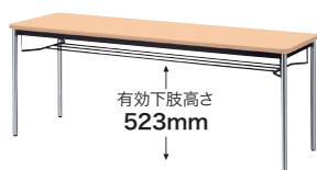
YB-S620 (棚付) WM/P W1800×D600×H700
