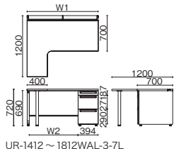
UR-1412 ~ 1812WAL-3-7L
