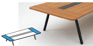
天板面寸法: W1225/1425/1625×D450mm
